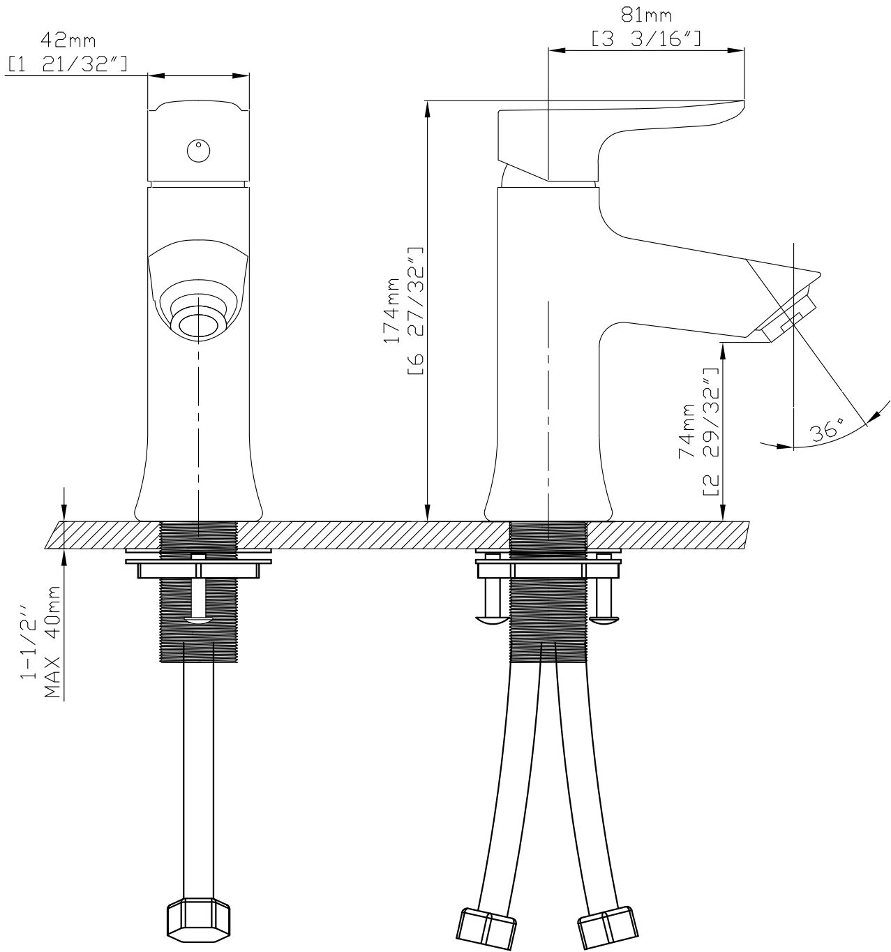
CRITICAL DIMENSIONS
