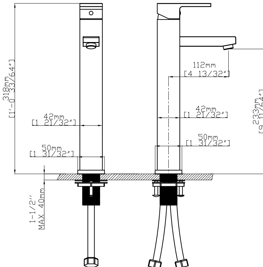
CRITICAL DIMENSIONS
