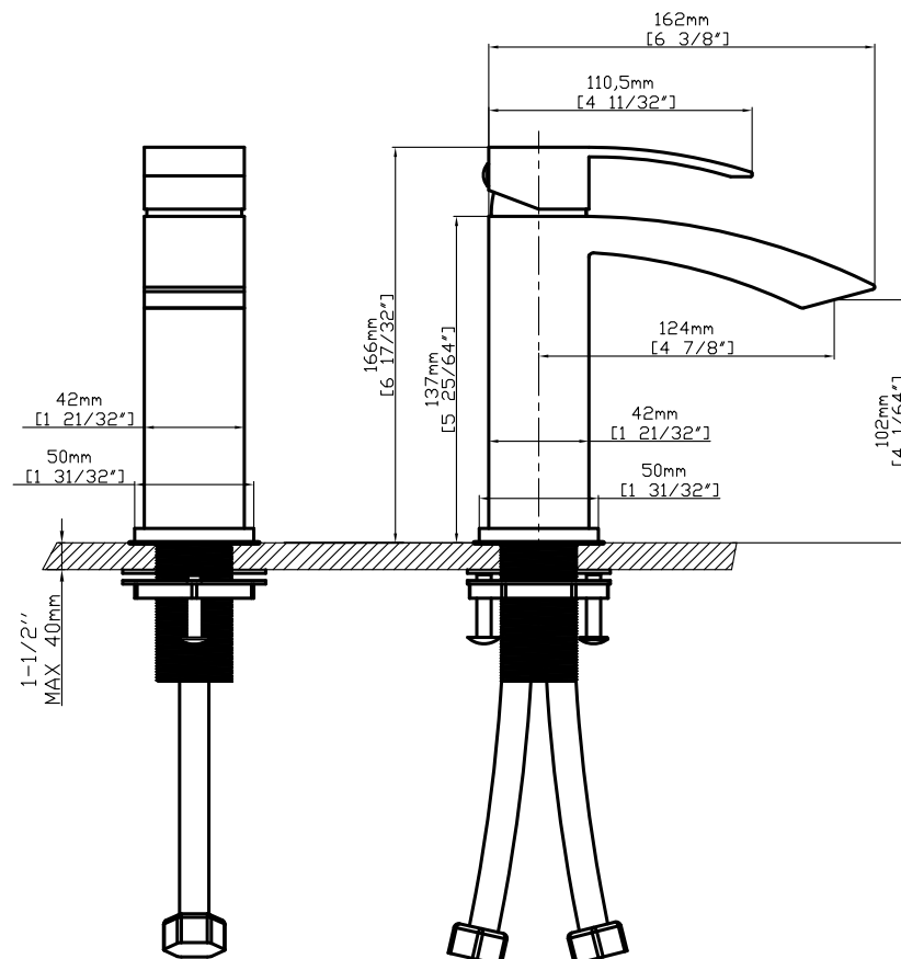
CRITICAL DIMENSIONS
